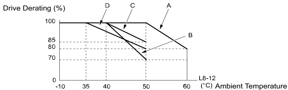
Figure 12: Ambient Temperature Derating Chart
